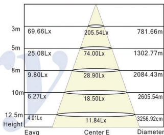
Illumination distance curve 50W
