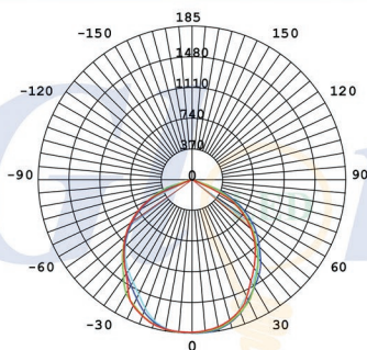
Light Distribution Curve 50W
