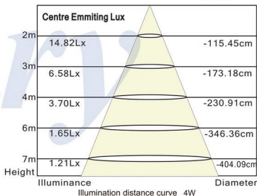
Light Distribution Curve 4W
