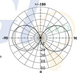
Light Distribution Curve 4W
